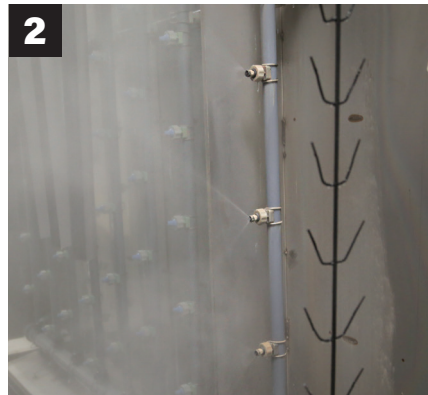
2 The product enters a heated cleaning stage to remove extrusion debris and fabrication oils.
