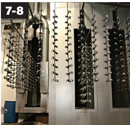
7-8 A 200 MPH air blast removes water drops from the pre-treated aluminum. A convection oven completes the dry-off process.
