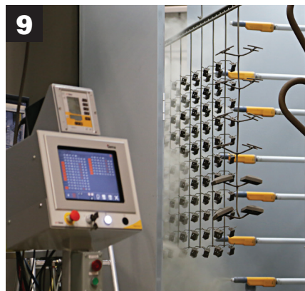
9 Powder is applied with 18 automated and 2 manual spray guns. Compressed process air is dried to -35°F Dew Point for superior adhesion.
